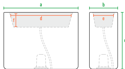
Smoov Planter 77_L
